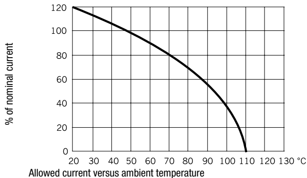
Allowed current versus ambient temperature
